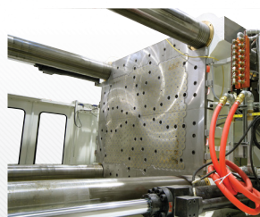
Magnetic Mold Clamps & Mold Changing Systems
