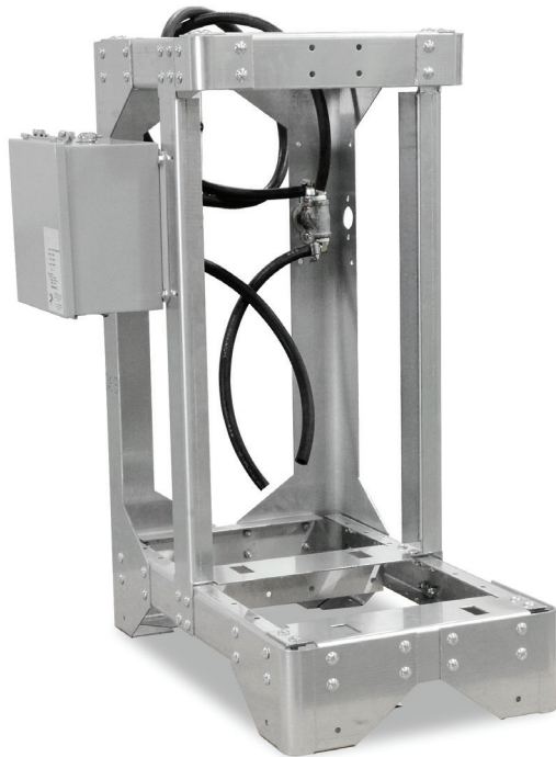
Stacking stand shown with Water Manifold and Optional Electrical Junction Box.
